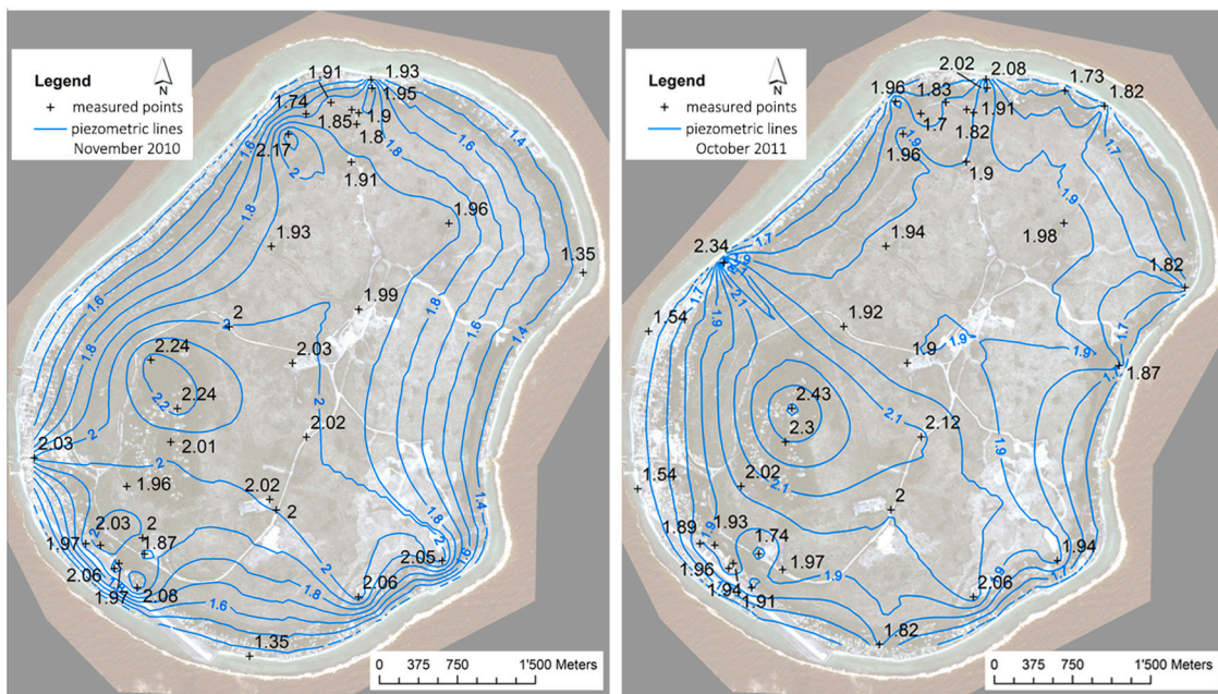
Figure 12. Piezometric maps of the groundwater heads measured in November 2010 and October 2011 (sea level 1.35 and 1.54 m, respectively).
