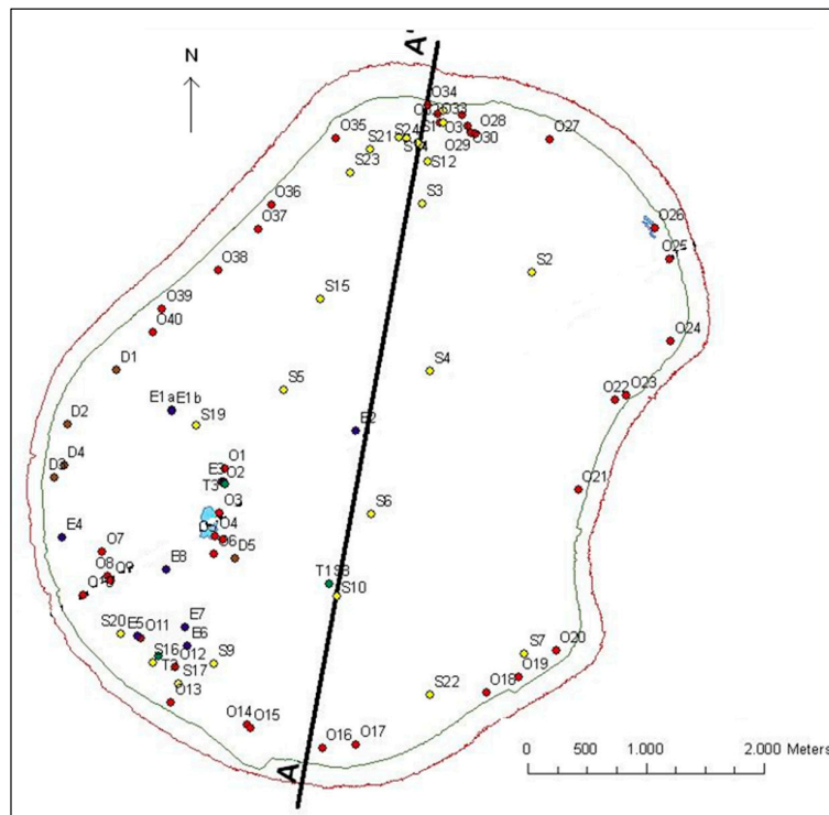
Figure 8. Section AA' trace and monitoring points present in the island.
