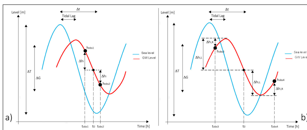
Figure 6. Groundwater level correction: Cases (i.) and (ii.) (a); and Cases (iii.) and (iv.) (b).
