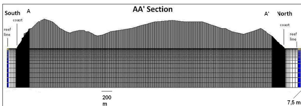
Figure 9. AA' section, black zones represent the most refined part of the model domain (1 m cells).
