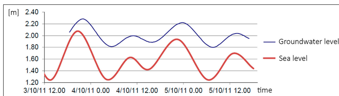
Figure 5. Sea and groundwater levels over a two-day observation period (compared to RL) in monitoring well S1 where the phreatic level varies within a range of 1.80–2.30 m every 6 h.
