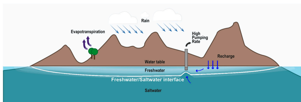
Figure 1. Small islands’ typical freshwater lens-shape over the brackish/salt water. The effect of a pumping well (upconing) is indicated.
