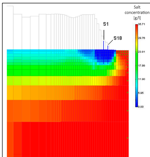
Figure 14. Concentration distribution of the calibrated model ( \text{kg}/\text{m}^3 ) simulated for November 2010 (zoom on the northern part of section AA); green dots indicate cells hosting the boundary condition.
