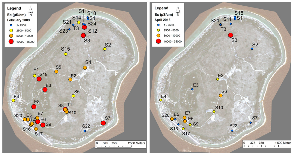
Figure 7. The 2009 and 2013 Electric Conductivity values at the water table into the Nauru aquifer.
