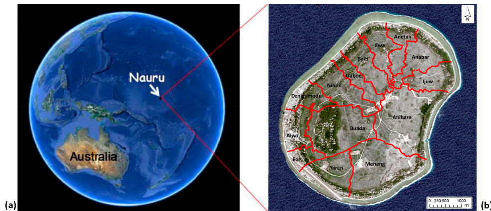
Figure 2. Nauru position at 0^{\circ}32' S and 166^{\circ}56' E (a); and aerial photo of the island in 2009 with its districts (b).
