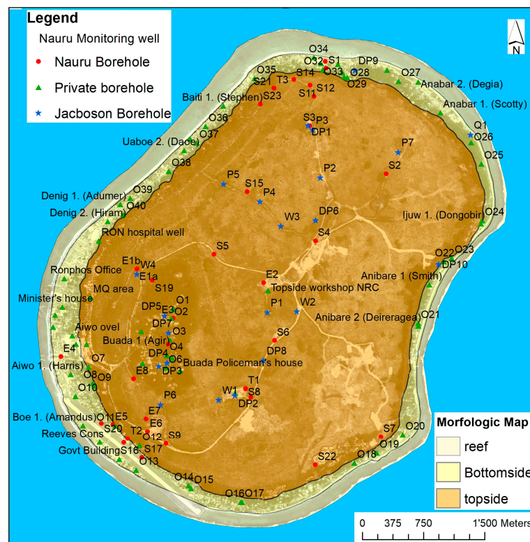
Figure 3. Reef, Bottomside and Topside of Nauru and location of wells and monitoring wells present in the island.
