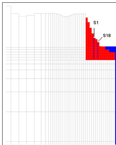
Figure 11. Calibrated hydraulic conductivity settings: sandy sediments (red) and limestone (white). In blue the constant head and constant concentration boundary conditions are indicated (zoom on the northern part of section AA’).
