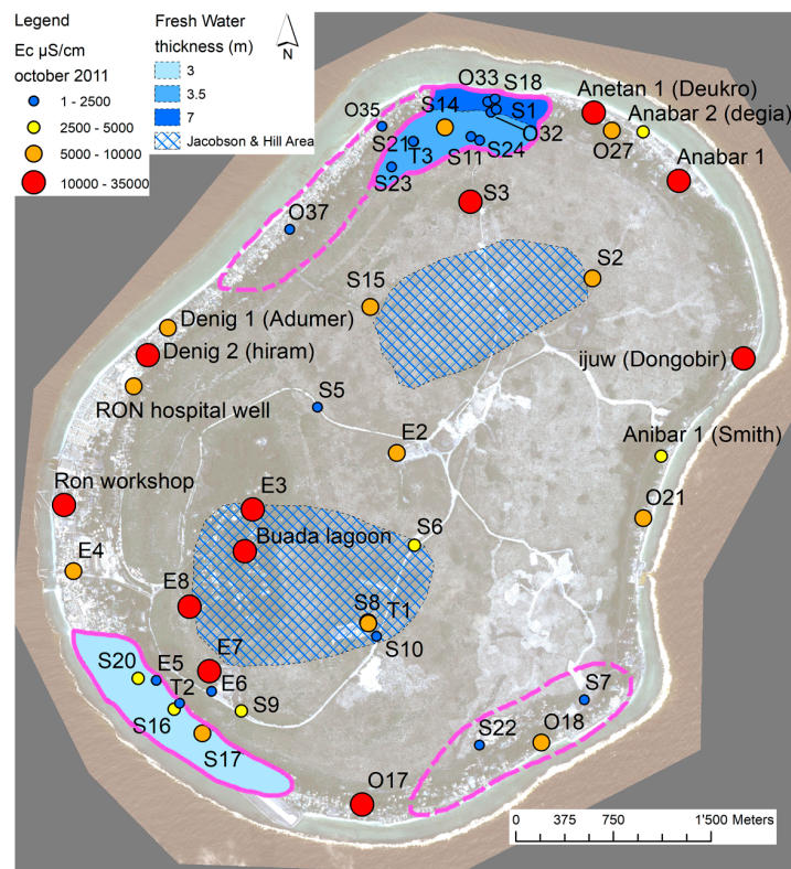
Figure 13. Results of the EC survey in monitoring wells and private wells (October 2011). Pink line indicates the most suitable areas for groundwater exploitation and the pink dashed one the potential suitable areas.
