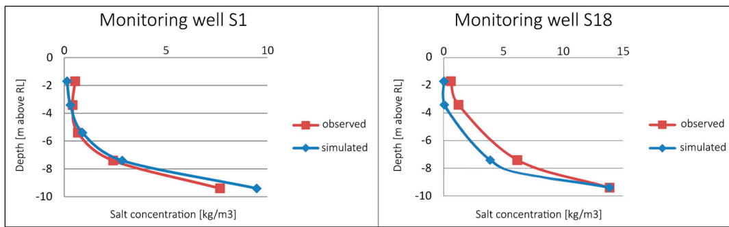
Figure 10. Observed vs simulated concentration values in monitoring wells S1 and S18.
