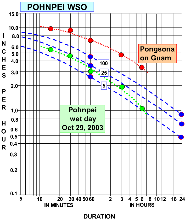
FIGURE 18 | Intensity-duration-frequency chart of selected return periods at the Pohnpei Weather Service Office (blue dots connected by blue dashed lines)
