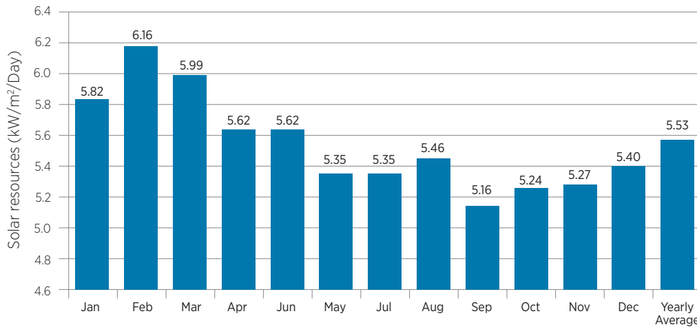
Figure 3: Majuro's average solar resource (kWh/m 2 /day)
