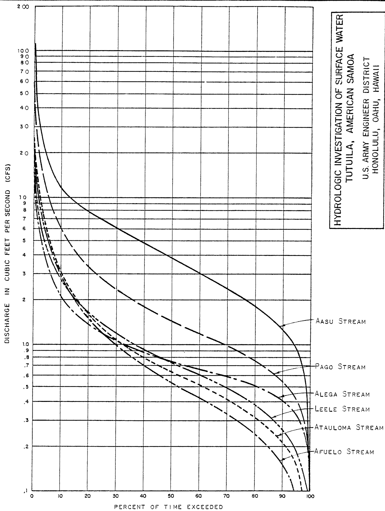
FLOW DURATION CURVES (COMPOSITE)
