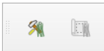
Fig. 13.1: GRASS toolbar
