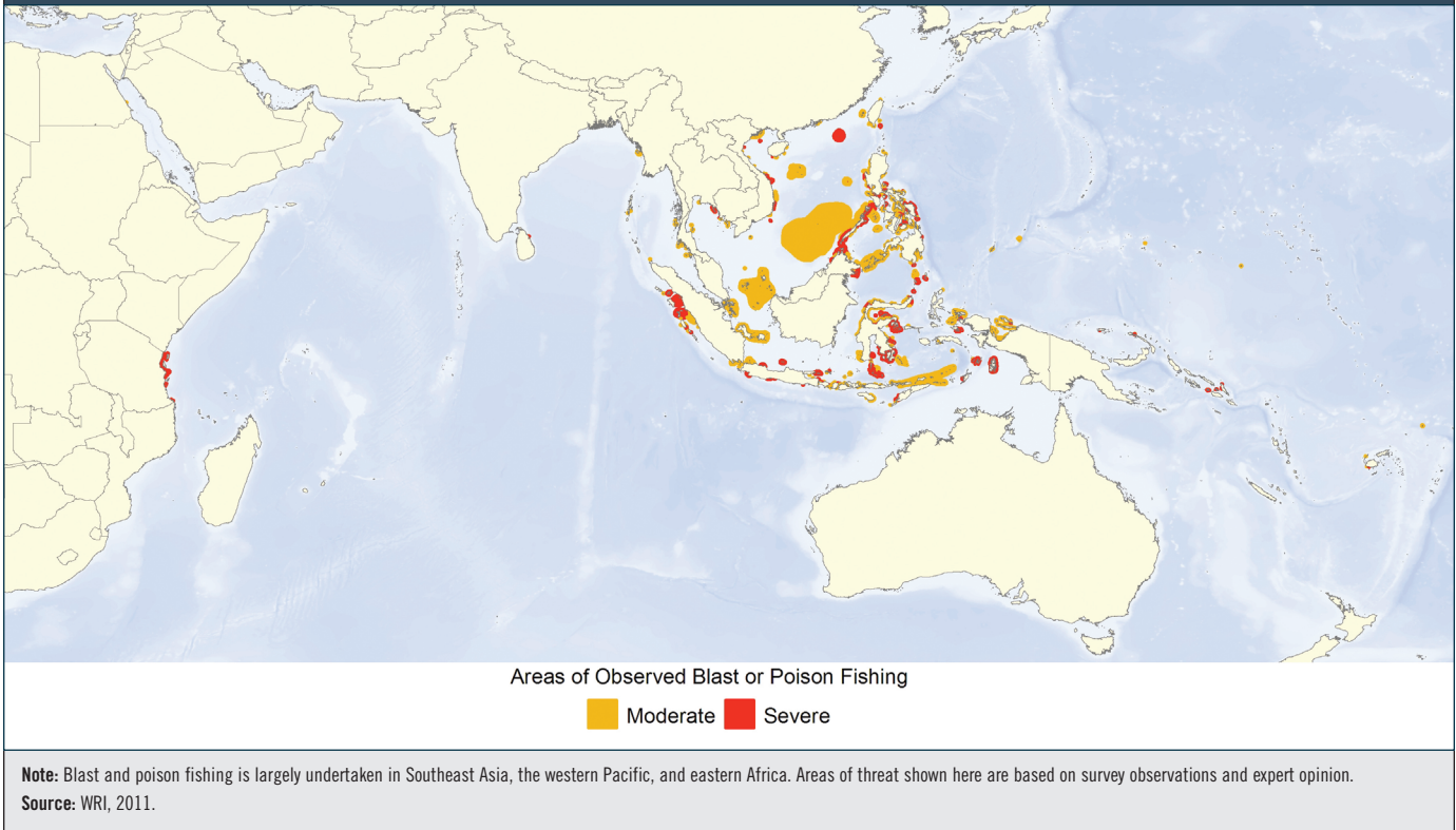
MAP 3.1. GLOBAL OBSERVATIONS OF BLAST AND POISON FISHING
