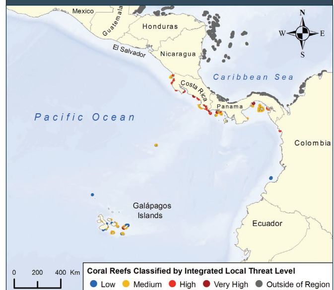
MAP 5.5b. REEFS AT RISK IN THE EASTERN PACIFIC
