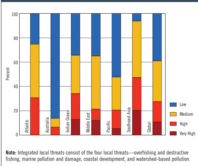
FIGURE ES-2. REEFS AT RISK FROM INTEGRATED LOCAL THREATS BY REGION
