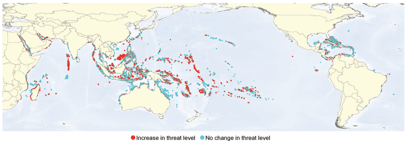
MAP 4.1. CHANGE IN LOCAL THREAT BETWEEN 1998 AND 2007
