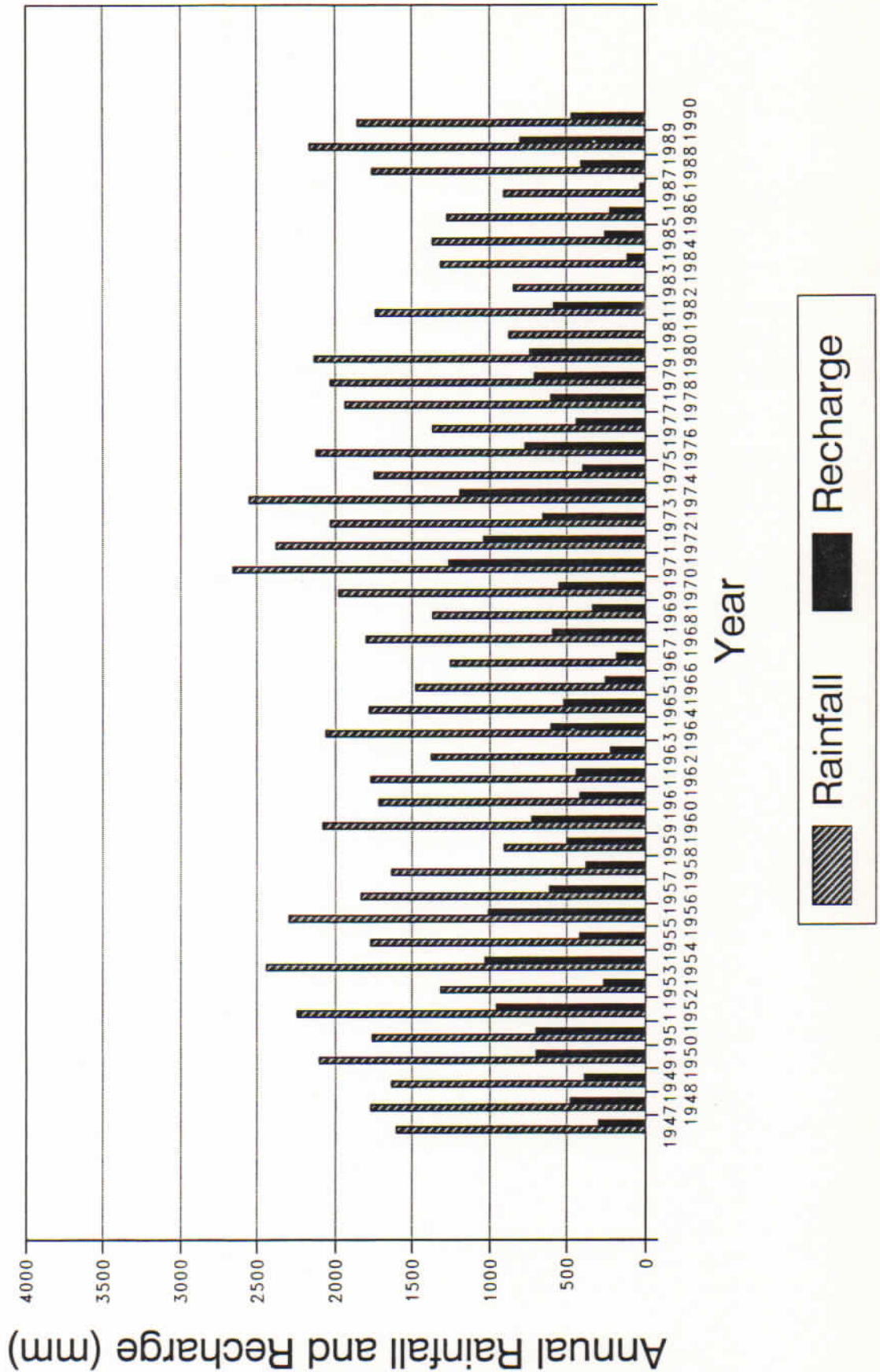
COMPARISON OF ANNUAL RAINFALL AND RECHARGE ON TONGATAPU, 1947-1990
