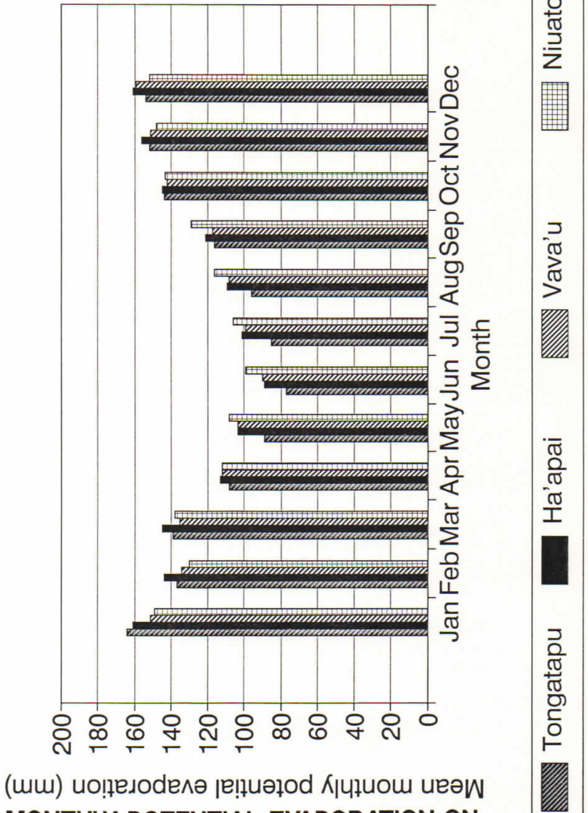
MEAN MONTHLY POTENTIAL EVAPORATION ON TONGATAPU, HA'APAI, VAVA'U AND NIUATOPUTAPU: 1947-1990
