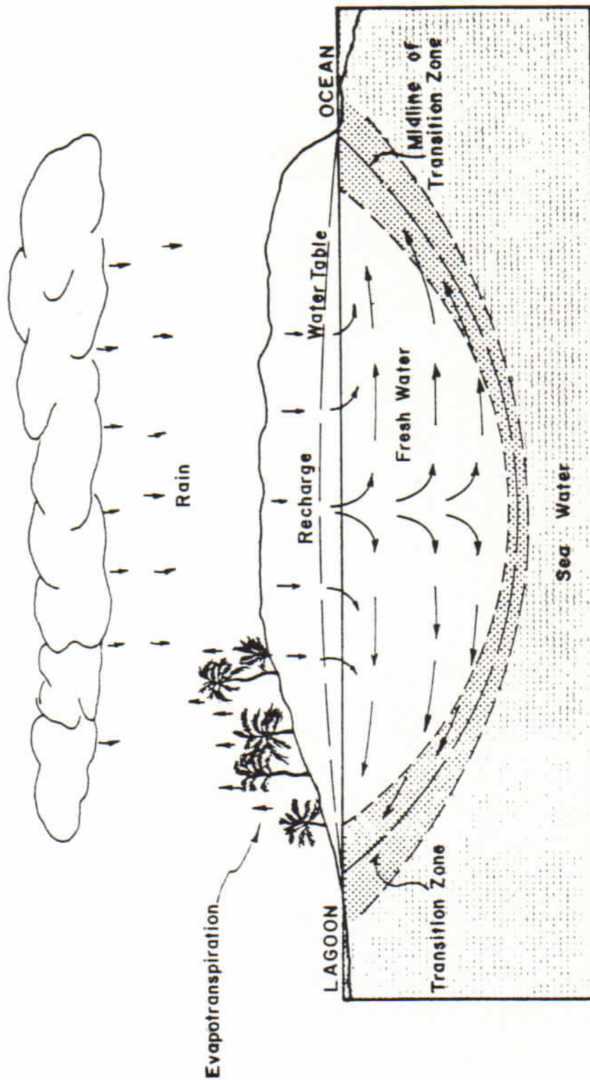
CROSS SECTION THROUGH A TYPICAL ATOLL
