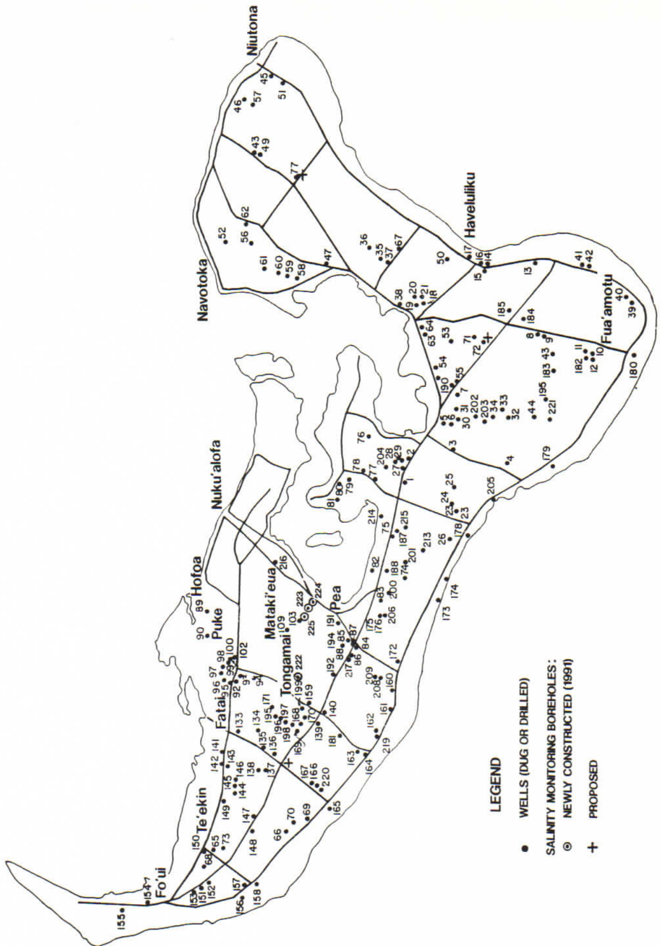
MAP OF TONGATAPU SHOWING LOCATION OF WELLS INCLUDED IN CENSUS
