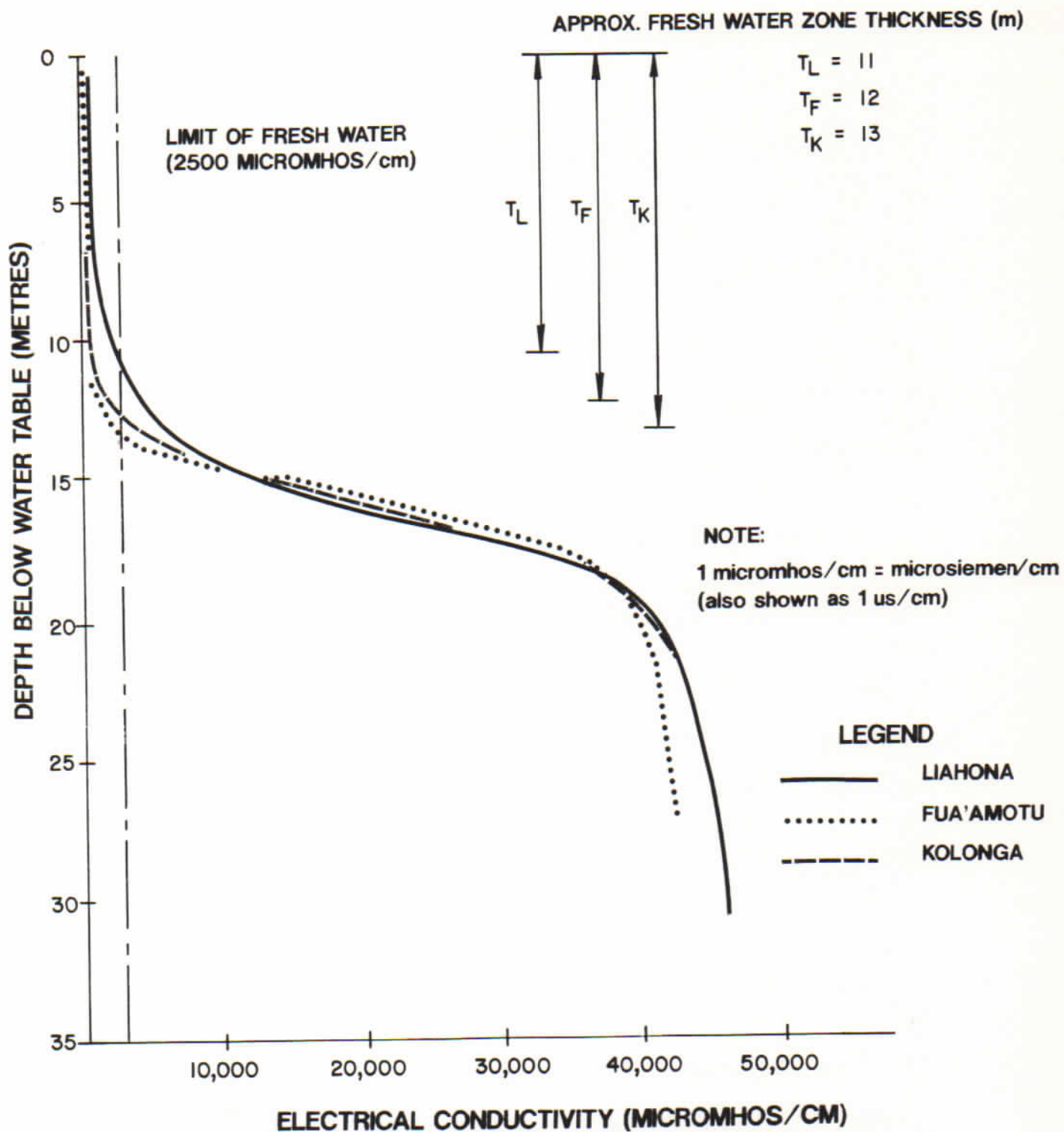
SALINITY PROFILES FROM DEEP MONITORING BORES ON TONGATAPU, NOVEMBER 1978
