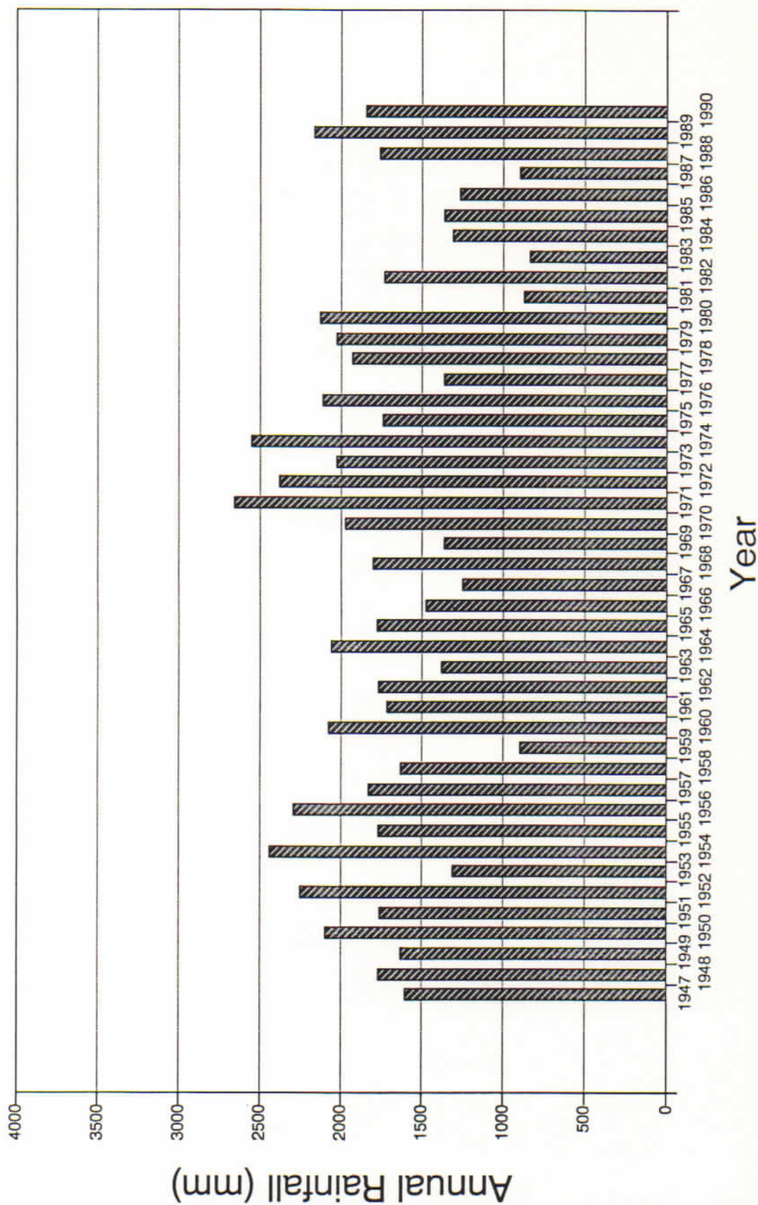
ANNUAL RAINFALL AT NUKU'ALOFA, TONGATAPU, 1947-1990
