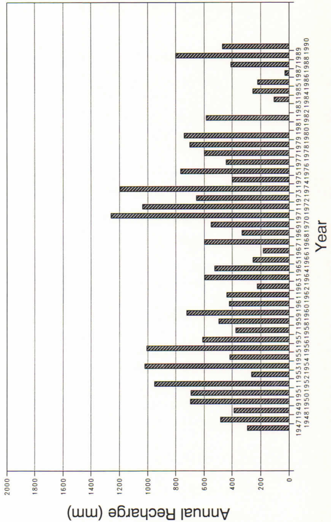
ANNUAL RECHARGE ON TONGATAPU, 1947-1990
