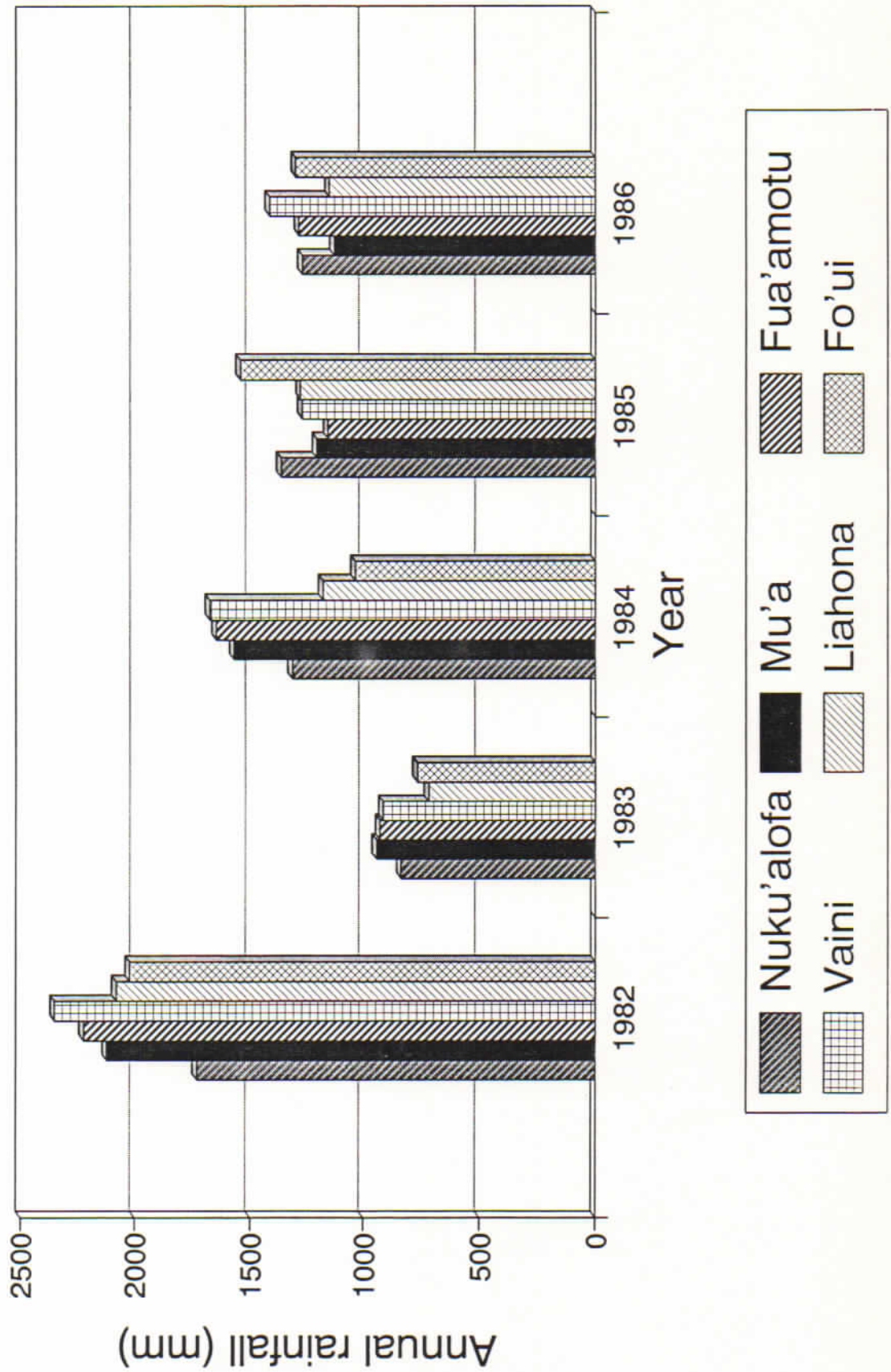
ANNUAL RAINFALL AT NUKU'ALOFA, MU'A, FUA'AMOTU, VAINI, LIAHONA AND FO'UI, 1982-1986
