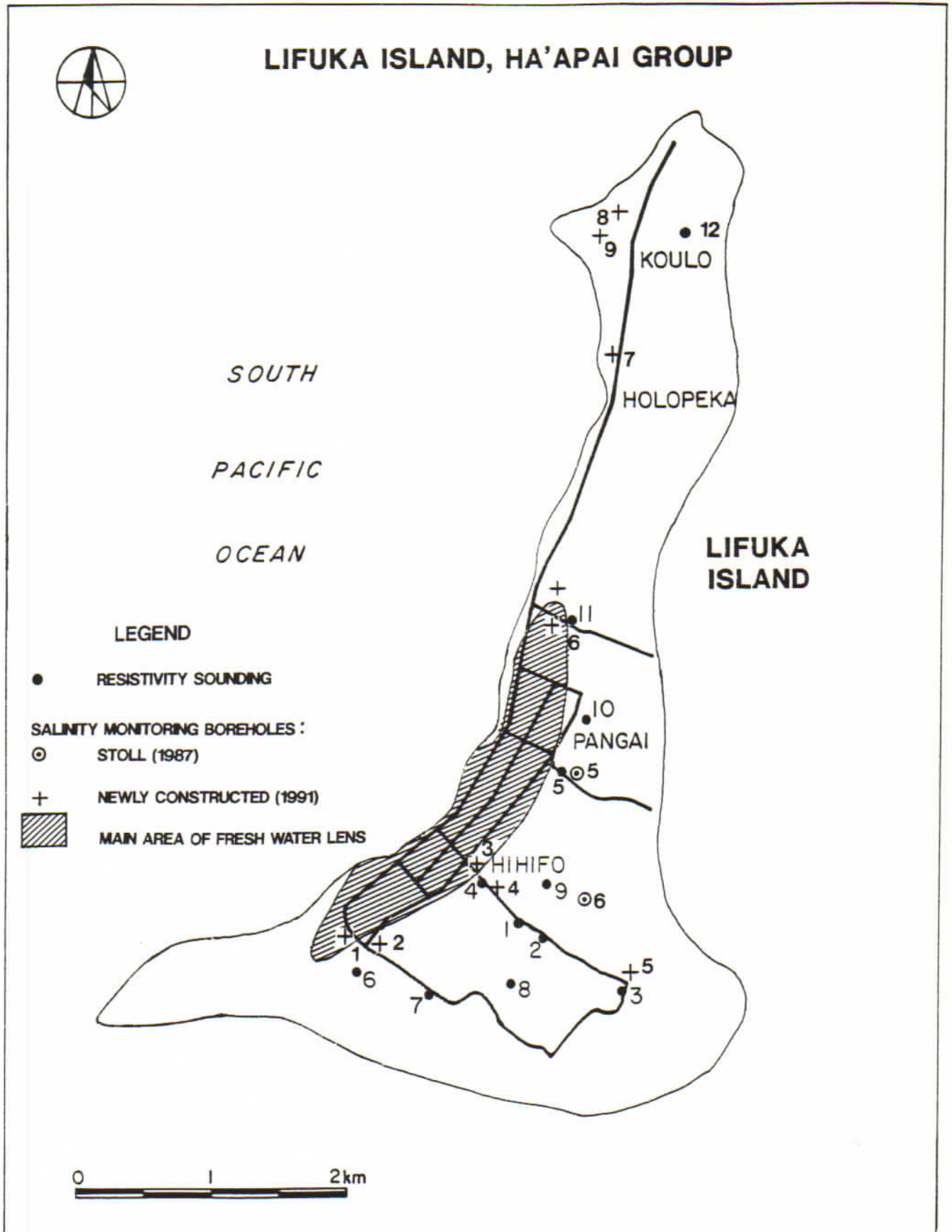
MAP OF LIFUKA SHOWING LOCATION OF ELECTRICAL RESISTIVITY SOUNDINGS, SALINITY MONITORING BOREHOLES AND MAIN AREA OF FRESHWATER LENS
