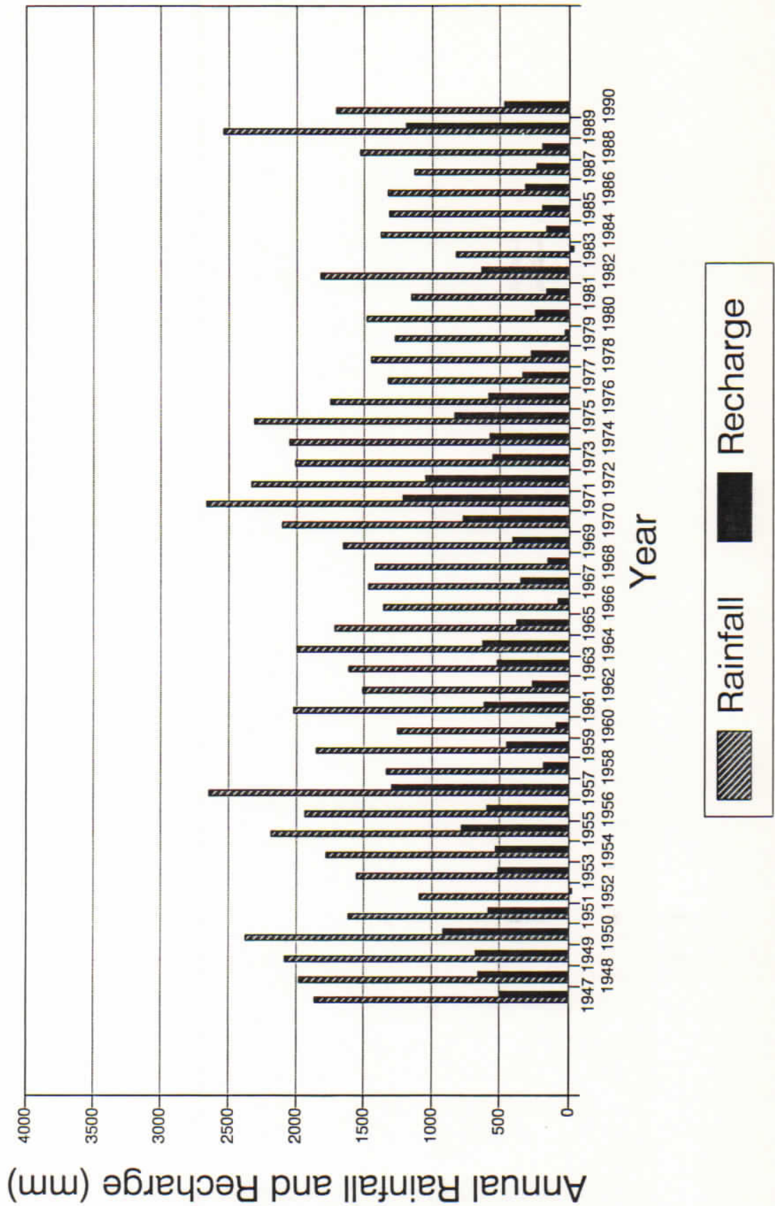
COMPARISON OF ANNUAL RAINFALL AND RECHARGE ON LIFUKA, HA'APAI, 1947-1990
