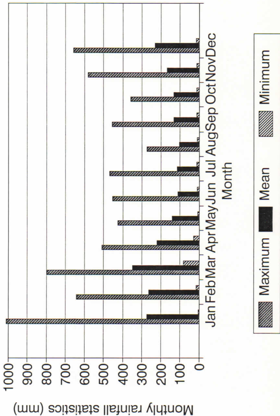
MAXIMUM, MEAN AND MINIMUM RAINFALL AT NEIAFU, VAVA'U FOR PERIOD 1947-1990
