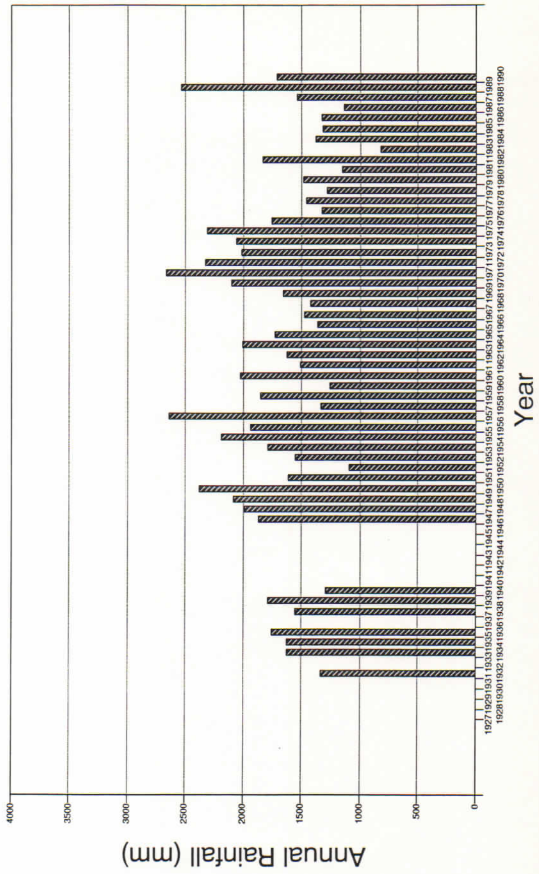
ANNUAL RAINFALL AT LIFUKA, HA'APAI, 1932-1990
