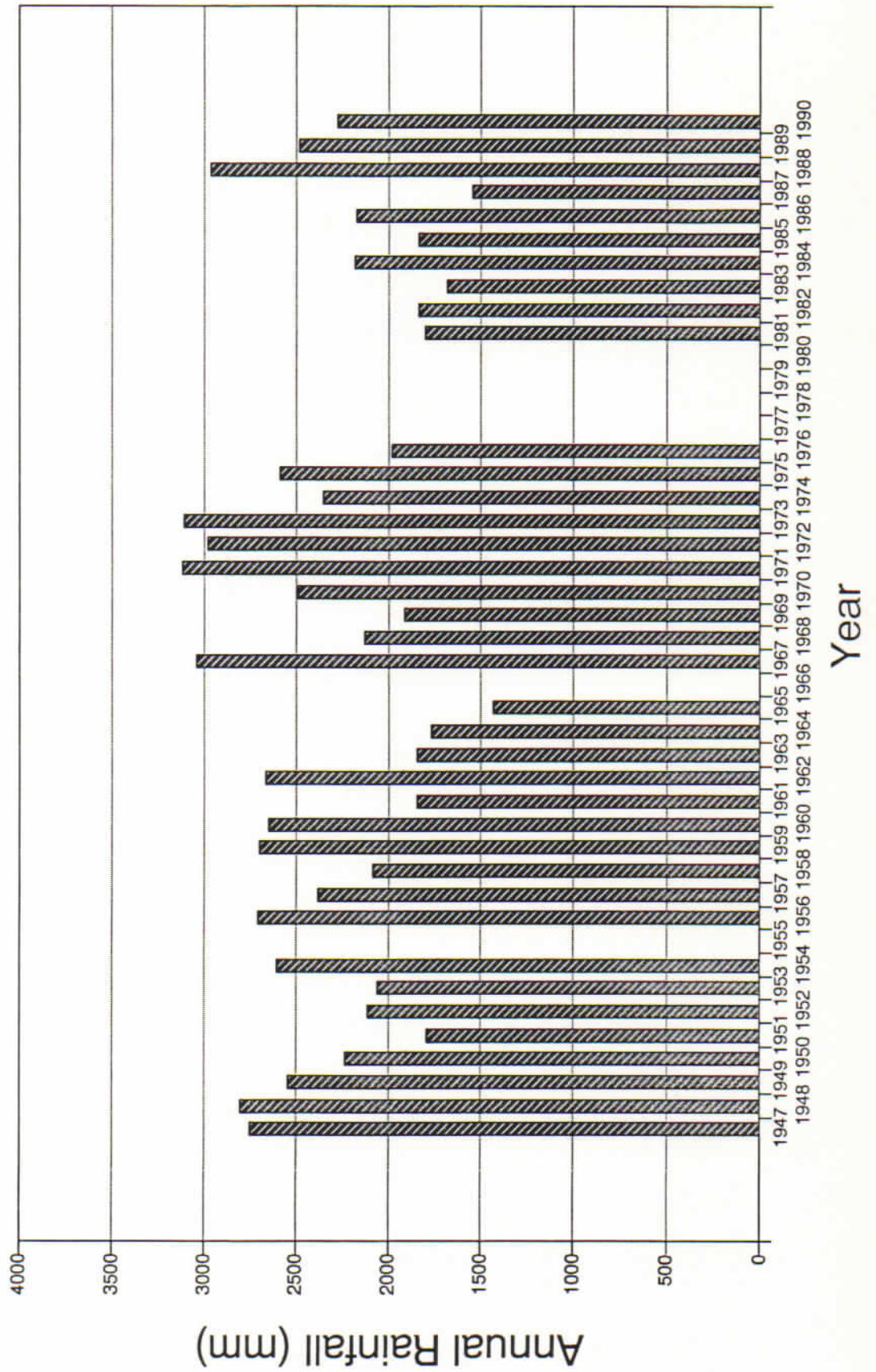
ANNUAL RAINFALL AT NIUTOPUTAPU, 1947-1990
