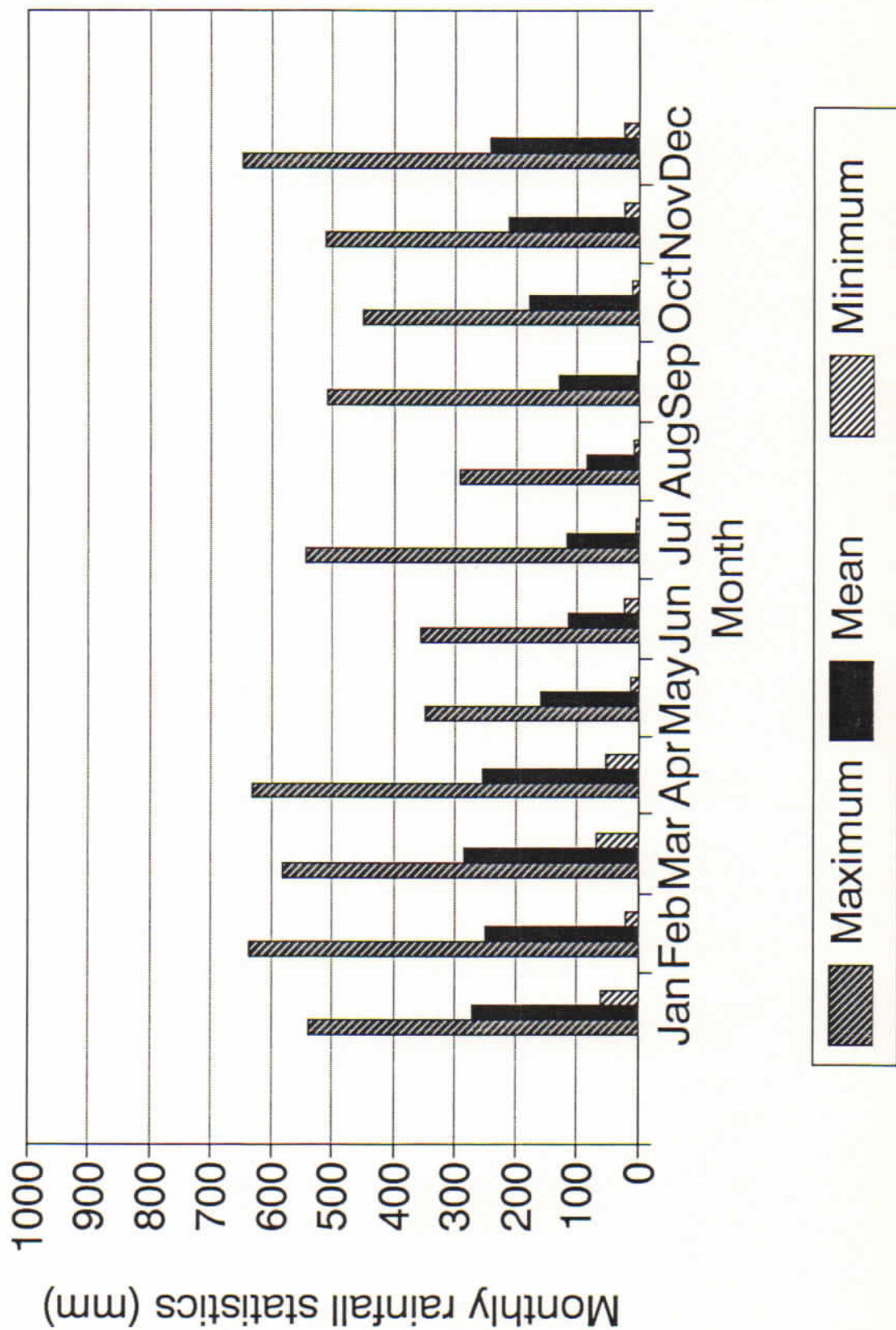
MAXIMUM, MEAN AND MINIMUM MONTHLY RAINFALL AT FALEHAU, NIUATOPUTAPU FOR PERIOD 1947-1990
