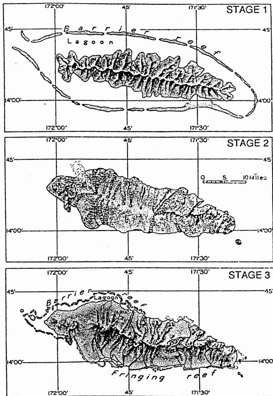
Figure 15. Outline of the island of Upolu, through time, as proposed by Stearns (1944). Stage 1 illustrates the proposed outlines of the island after extensive erosion of the shield building lavas. Stage 2 illustrates the outline of the island after the barrier reefs were drowned and volcanism was renewed. Stage 3 illustrates the present configuration of the island and the partial development of fringing and barrier reefs around the margin of the island.
