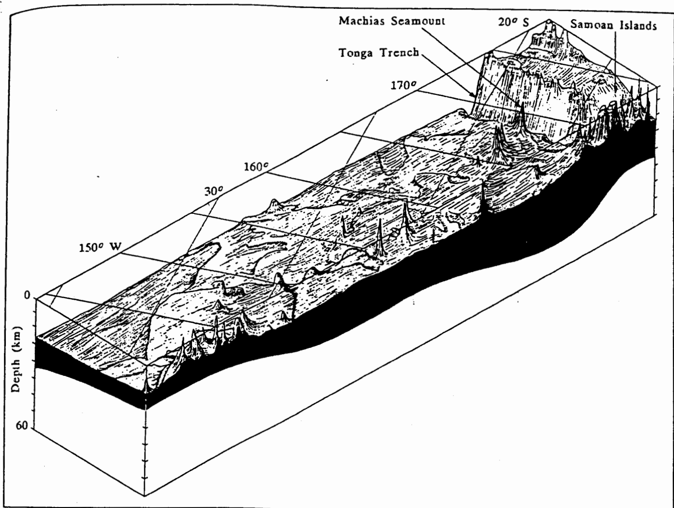
Figure 35. Cross-sectional view of the Samoan and Austral-Cook seamount and island chains, showing their proximity to the Tongan Trench. The view point is near the equator looking south toward the Tongan Trench. The black shading was added by the artist and does not reflect crustal structure. Drawing by Dick Rhodes.
