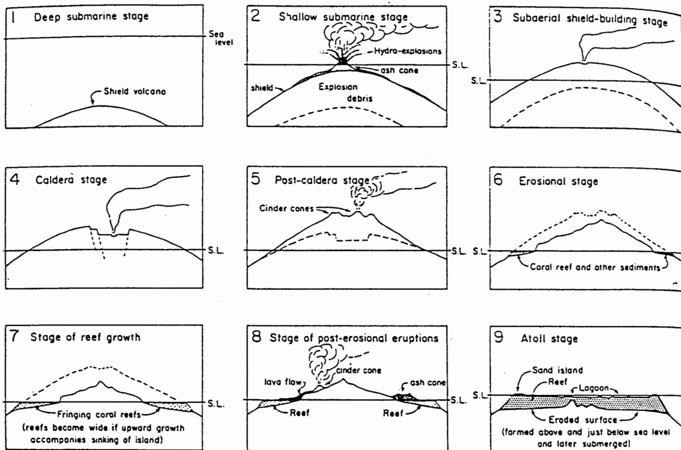
Figure 30. Stages of volcanism observed from the Hawaiian chain (from Macdonald and Abbott, 1970).
