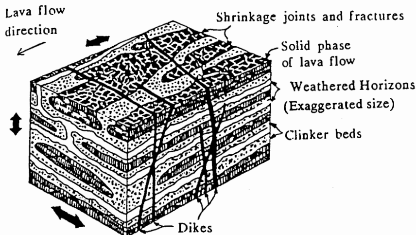
Figure 28. Block diagram illustrating the complex geologic relationships in volcanic landscapes. A complex interfingering of flow units and volcanoclastic units can be present. Dikes, intruding the edifice, can complicate the hydrology by acting as vertical barriers to water movement. (Figure modified from Hunt and others, 1988).
