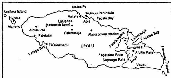
Figure 11. Site location map for localities in Upolu referenced in the text.
