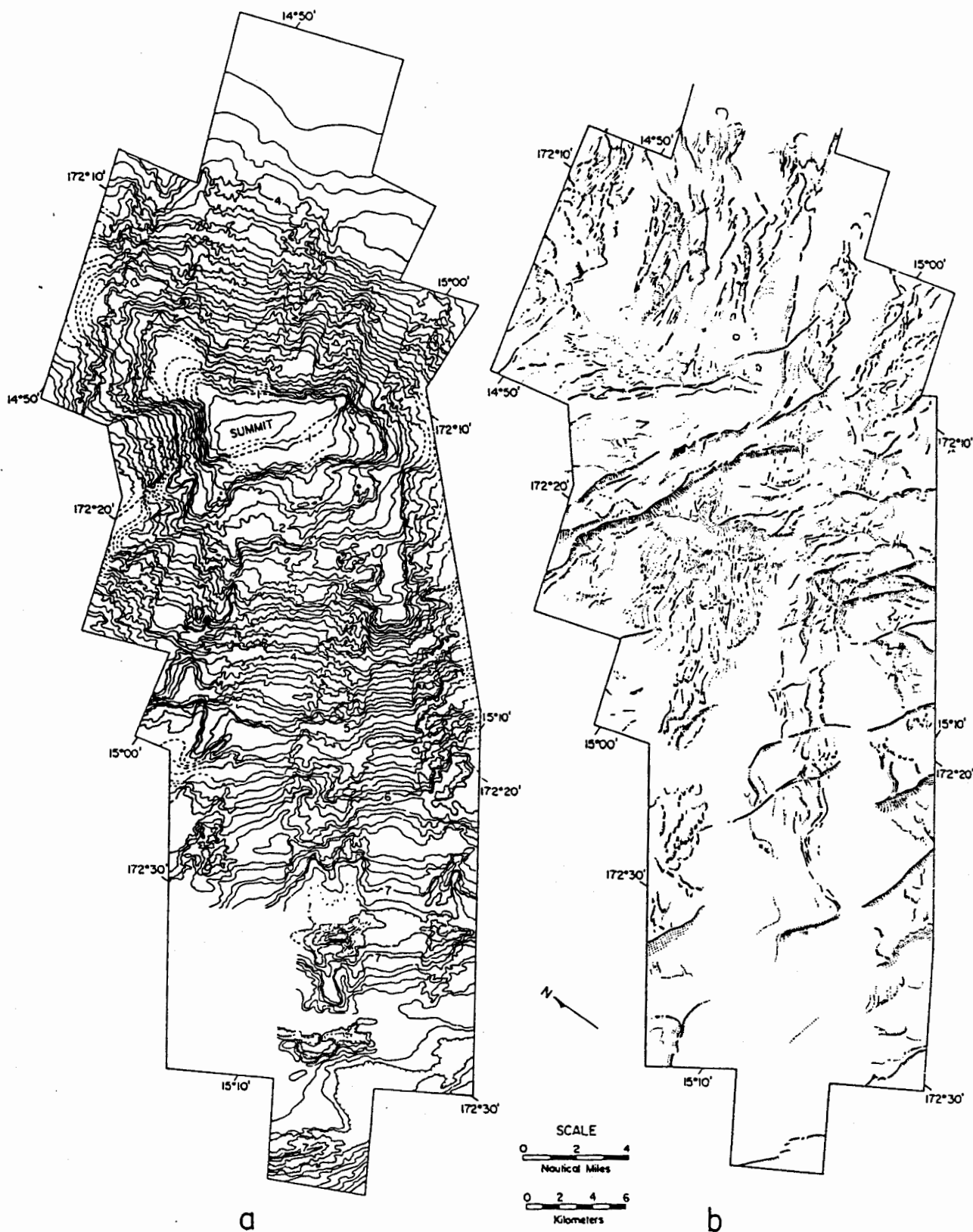
Figure 12. Bathymetric map and sketch map of Machias Seamount showing faulted structure of the seamount. The faulting is believed to be a consequence of deformation of the Pacific plate at the lip of the Tonga Trench subduction zone. (Figure from Coulbourn et al., 1989).
