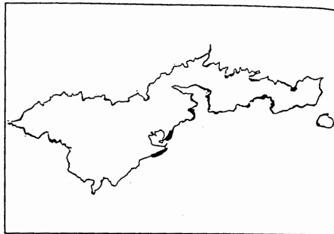
Figure 19. Map of the island of Tutuila, showing the locations of the modern reef edge as mapped by Stearns (1944) and Wingert (1981).
