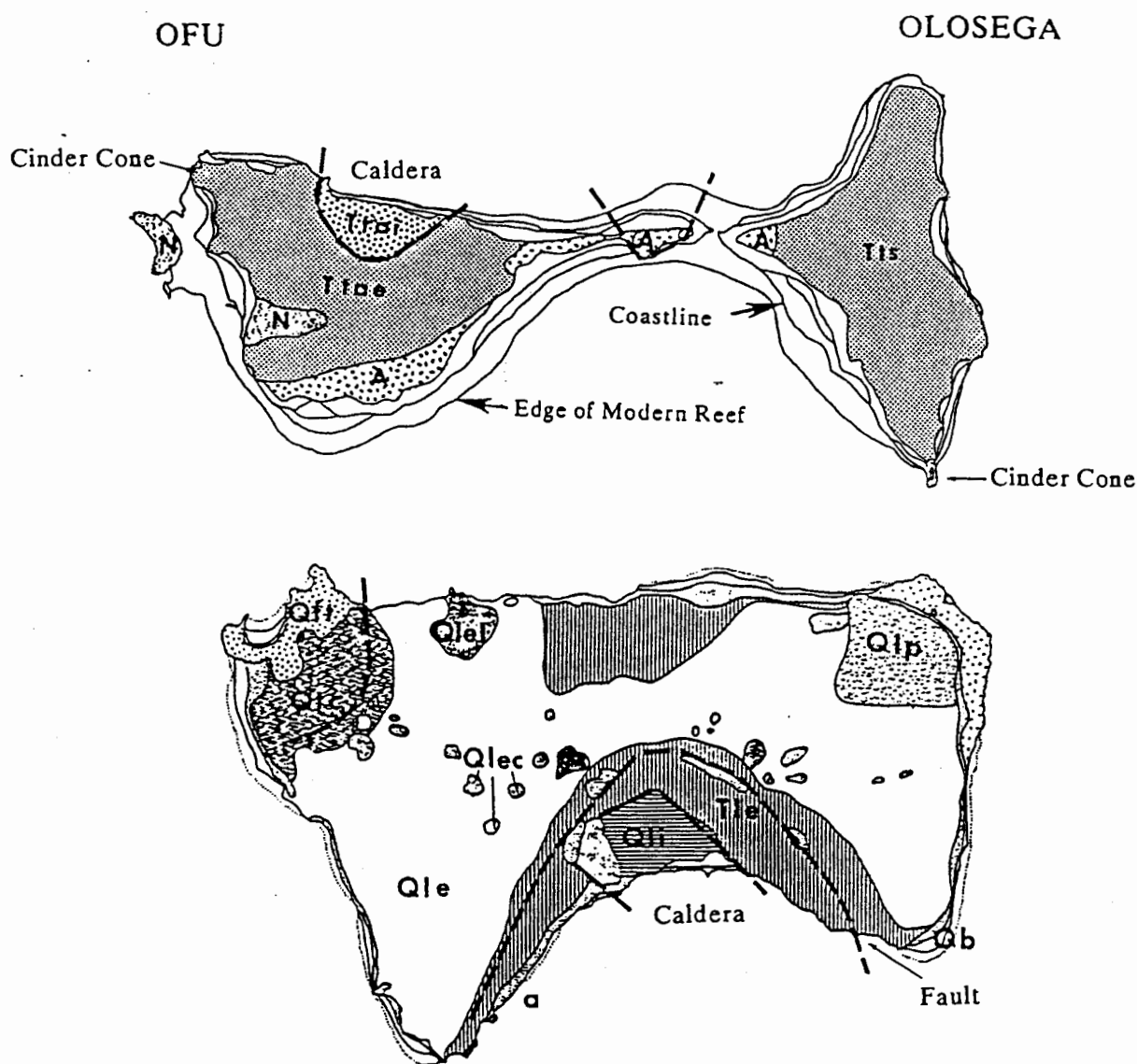
Figure 17. Geologic maps of the Manua Group, based upon maps by Stice and McCoy (1968) and later republished by Wingert (1981). The islands of Ofu and Olosega are shown at top. The island of Tau is shown at the bottom of the figure. In the upper figure the map symbols (in ascending stratigraphic order) are: A = Asaga Formation (the oldest mapping unit of Pliocene age), Ttai = ponded flows of the Tuafanua Formation, Tts = Tuafanua Formation flows, Ttae = flows of the Tuafanua Formation, N = tuffs of the Nu'u Formation. The remaining units, which are not separately designated are Quaternary sediments. The geologic map of Tau is shown in the lower figure. The map symbols used represent the following map units (in ascending order): Tle = lava flows of the Lata Formation, Qli = intra-caldera member of Lata Formation, Qle = post-caldera volcanics of the Lata Formation, Qtc = ash, tuff, and olivine basalt of the Tunoa Formation, Qlc = ponded lavas of Luatele Formation, Qlp = flows of Luatele Formation, Qft = Faleasao Tuff Formation, Qa = alluvium, Qb = modern beach sediments. The remaining units which are not separately designated are Quaternary sediments.
