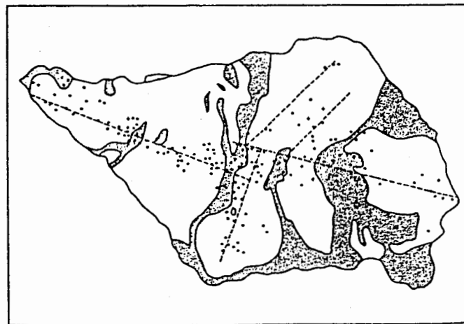
Figure 6. Map of Savaii showing the location of historic lava flows, cones, and the inferred rift zones. Based upon geologic map of Kear and Wood (1959). The dots represent cones and the dashed lines are inferred rift zones.
