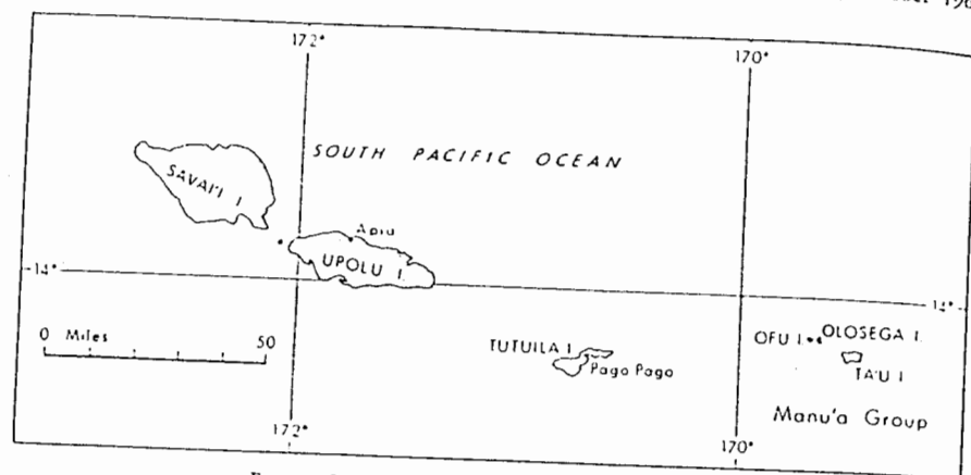
FIG. 1. Location map of the Manu'a Islands, Samoa.
