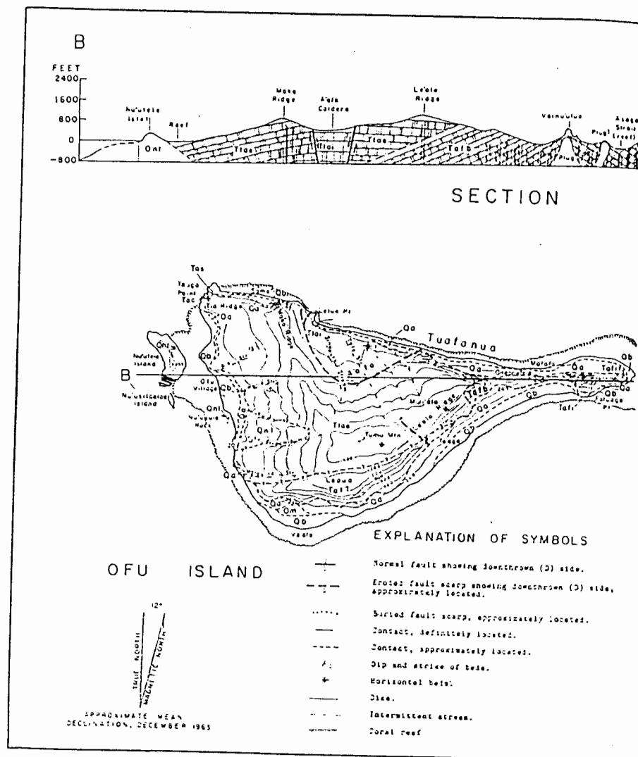
FIG. 8. Detailed geologic map and cross section of Ofu and Olosega islands.
